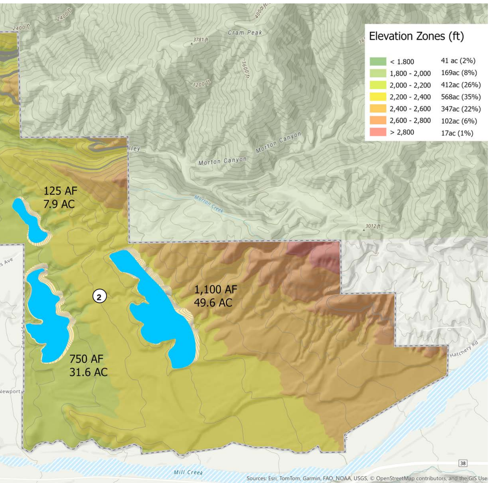
Figure 11. Conceptual Reservoir Opportunities consider placements that maximize gravity to function in concert with existing SWP facilities at elevations 2310 and 1938 feet.
