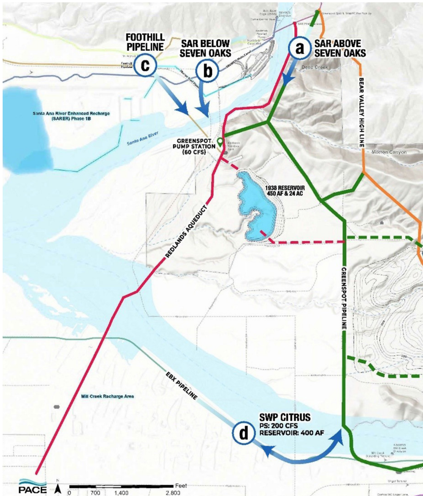
Figure 12. Water Source Opportunities
