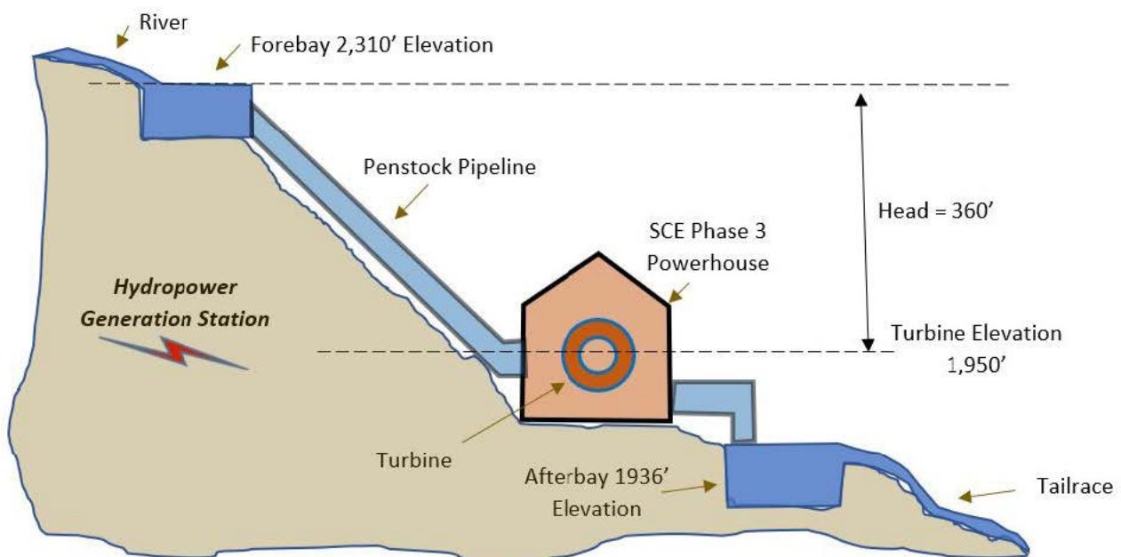
Figure 10. Hydropower Generation at Santa Ana River Powerhouse 3
