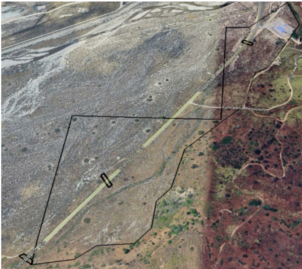
Figure 24. Potential movement corridors for San Bernardino kangaroo rat
