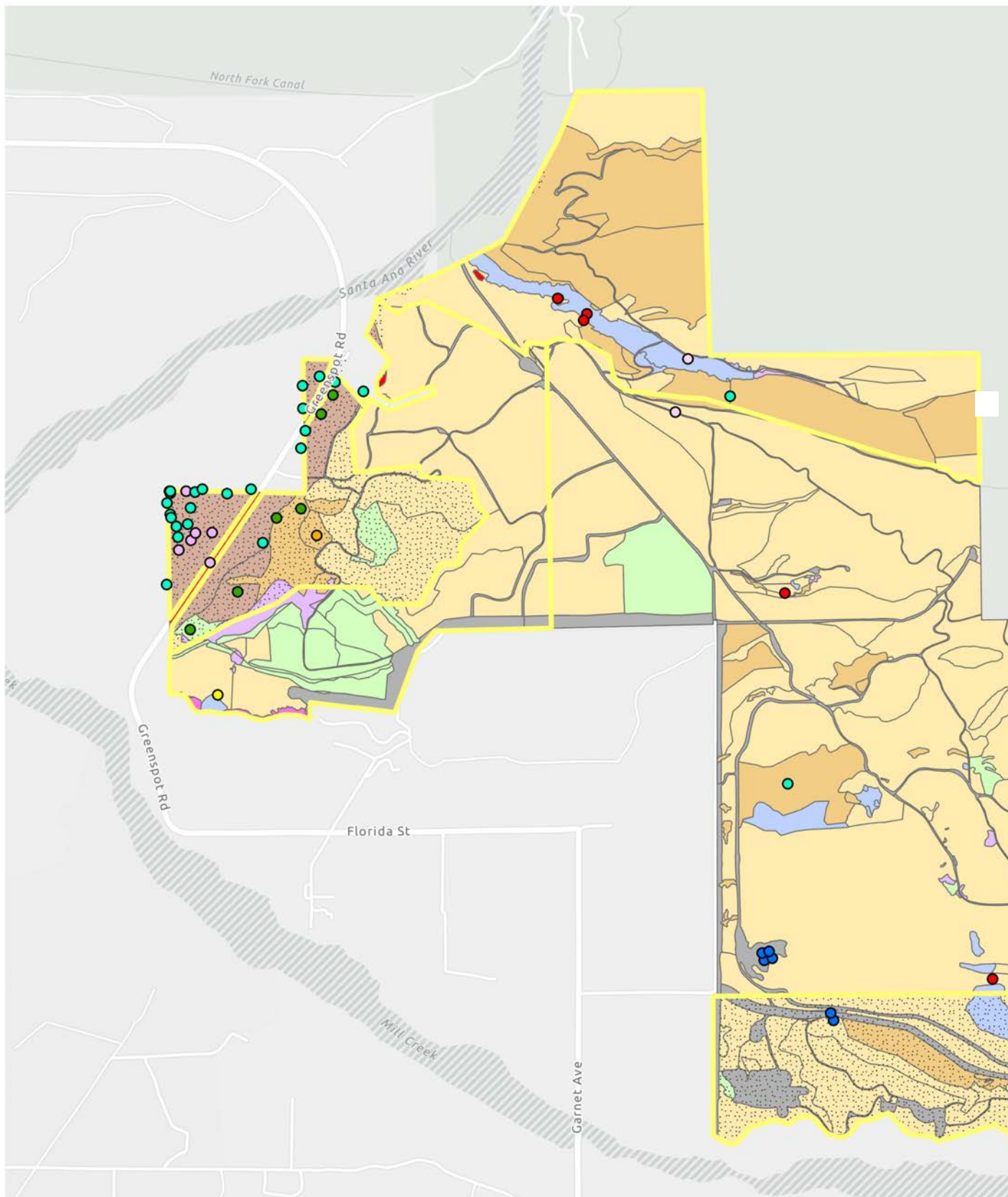
Figure 19. Plant communities and special status species observed on Sunrise Ranch property
