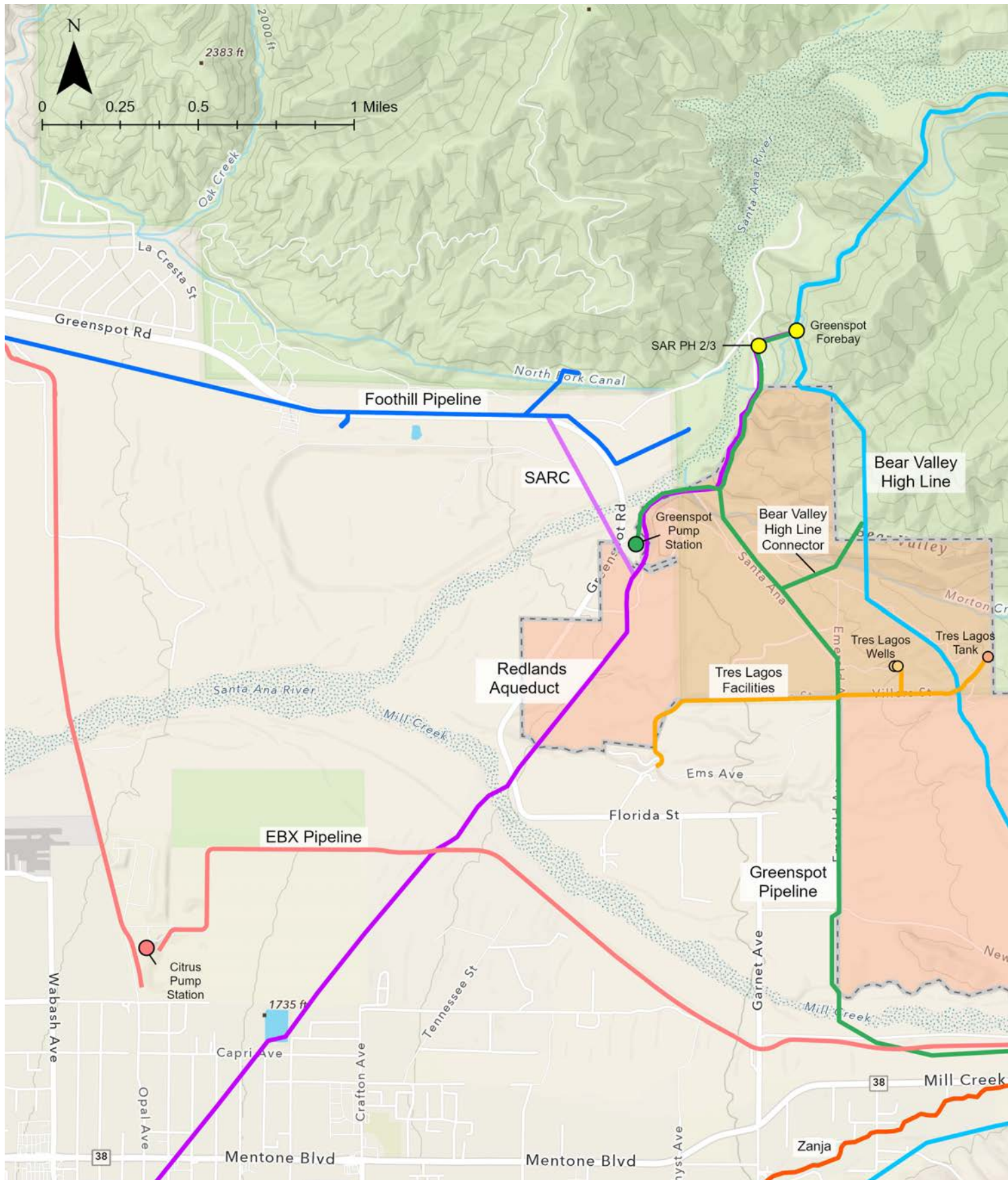
Figure 7. Existing Water Infrastructure at Sunrise Ranch and Vicinity
