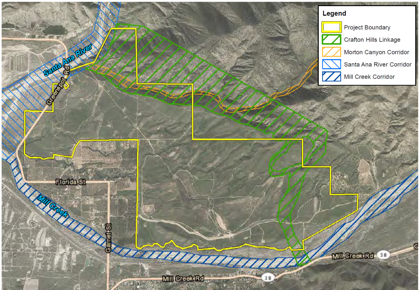
Figure 23. Localized wildlife movement per the 2014 FEIR Harmony Development review; Illustration based on field observations and area topography
