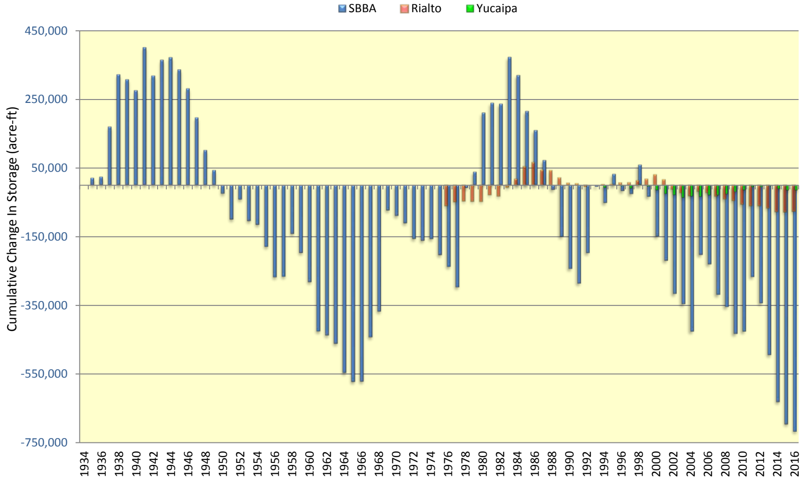
Figure 7. Comparison of SBBA, Yucaipa and Rialto-Colton Basin Cumulative Change in Storage
